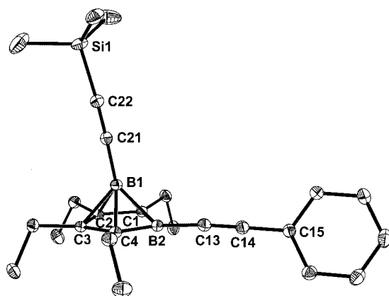
Figure 3. Molecular structure of 8 ; hydrogen atoms omitted for clarity; thermal ellipsoids are shown at 40% probability; selected bond lengths [Å] and angles [°]: B(1)–C(1) 1.723(2), B(1)–C(2) 1.735(2), B(1)–C(3) 1.734(2), B(1)–C(4) 1.731(2), B(1)–B(2) 1.833(2), B(2)–C(1) 1.532(2), B(2)–C(4) 1.532(2), C(1)–C(2) 1.455(2), C(2)–C(3) 1.440(2), C(3)–C(4) 1.452(2), B(2)–C(13) 1.536(2), C(13)–C(14) 1.207(2), C(14)–C(15) 1.438(2), B(1)–C(21) 1.522(2), C(21)–C(22) 1.205(2); C(21)–B(1)–B(2) 142.49(10), C(13)–B(2)–B(1) 132.30(10), C(14)–C(13)–B(2) 175.39(13), C(13)–C(14)–C(15) 178.79(13), C(22)–C(21)–B(1) 177.62(12), C(21)–C(22)–Si(1) 175.45(12)
