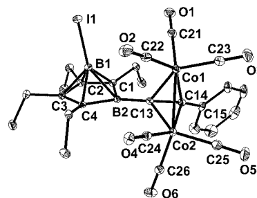
Figure 4. Molecular structure of 9 ; hydrogen atoms omitted for clarity; thermal ellipsoids are shown at 40% probability; selected bond lengths [Å] and angles [°]: I(1)–B(1) 2.121(2), B(1)–C(1) 1.712(3), B(1)–C(2) 1.712(3), B(1)–C(3) 1.718(3), B(1)–C(4) 1.705(3), B(1)–B(2) 1.826(3), B(2)–C(1) 1.537(3), B(2)–C(4) 1.537(3), C(1)–C(2) 1.458(3), C(2)–C(3) 1.443(3), C(3)–C(4) 1.456(3), B(2)–C(13) 1.554(3), C(13)–C(14) 1.348(3), C(14)–C(15) 1.465(3), Co(1)–Co(2) 2.483(4), Co(1)–C(13) 1.537(3), Co(1)–C(14) 1.952(2), Co(2)–C(13) 1.990(2), Co(2)–C(14) 1.976(2); B(2)–B(1)–I(1) 140.7(2), C(13)–B(2)–B(1) 130.5(2), C(14)–C(13)–B(2) 141.1(2), C(13)–C(14)–C(15) 140.1(2)
