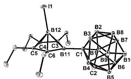
Figure 5. Molecular structure of 10 ; hydrogen atoms omitted for clarity; thermal ellipsoids are shown at 40% probability; selected bond lengths [Å] and angles [°]: I(1)–B(12) 2.125(2), B(12)–C(3) 1.708(2), B(12)–C(4) 1.731(2), B(12)–C(5) 1.731(2), B(12)–C(6) 1.710(2), B(11)–B(12) 1.817(2), B(11)–C(3) 1.543(2), B(11)–C(6) 1.541(2), B(11)–C(1) 1.595(2), C(1)–C(2) 1.687(2), B(11)–B(12)–I(1) 141.46(10), C(1)–B(11)–B(12) 132.04(12)
