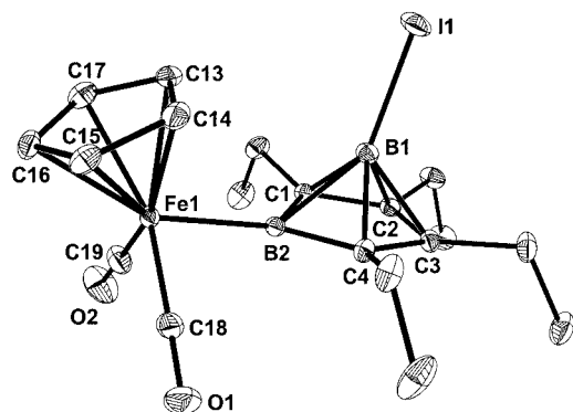
Figure 2. Molecular structure of 4 ; hydrogen atoms omitted for clarity; thermal ellipsoids are shown at 40% probability; selected bond lengths [Å] and angles [°]: I(1)–B(1) 2.135(2), B(1)–C(1) 1.692(2), B(1)–C(2) 1.711(2), B(1)–C(3) 1.709(2), B(1)–C(4) 1.689(3), B(1)–B(2) 1.841(3), B(2)–C(1) 1.547(2), B(2)–C(4) 1.547(2), C(1)–C(2) 1.460(2), C(2)–C(3) 1.431(2), C(3)–C(4) 1.468(2), Fe(1)–B(2) 2.069(2), Fe(1)–C(19) 1.739(2), Fe(1)–C(18) 1.742(2), Fe(1)–C cp 2.094–2.116(2), O(1)–C(18) 1.150(2), O(2)–C(19) 1.151(2); B(2)–B(1)–I(1) 142.91(11), B(1)–B(2)–Fe(1) 133.48(11), C(19)–Fe(1)–C(18) 92.59(10), C(19)–Fe(1)–B(2) 86.26(8), C(18)–Fe(1)–B(2) 85.03(8), O(1)–C(18)–Fe(1) 178.7(2), O(2)–C(19)–Fe(1) 178.6(2)
