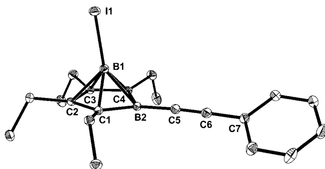
Figure 1. Molecular structure of 2a ; hydrogen atoms omitted for clarity; thermal ellipsoids are shown at 40% probability; selected bond lengths [Å] and angles [°]: I(1)–B(1) 2.139(2), B(1)–C(1) 1.714(3), B(1)–C(2) 1.722(3), B(1)–C(3) 1.714(3), B(1)–C(4) 1.706(3), B(1)–B(2) 1.825(3), B(2)–C(1) 1.537(3), B(2)–C(4) 1.532(3), C(1)–C(2) 1.453(3), C(2)–C(3) 1.446(2), C(3)–C(4) 1.459(3), B(2)–C(5) 1.529(3), C(5)–C(6) 1.211(3), C(6)–C(7) 1.435(3); B(2)–B(1)–I(1) 143.3(1), C(5)–B(2)–B(1) 131.2(2), C(6)–C(5)–B(2) 177.0(2), C(5)–C(6)–C(7) 178.3(2)
